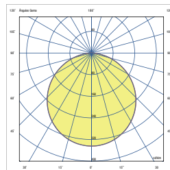
Galaxy LED IP65 40W 3200lm 120°
