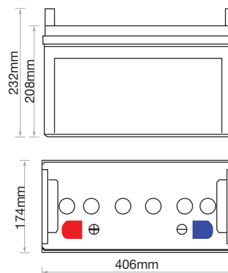
Bateria 120Ah/ Battery 120Ah
